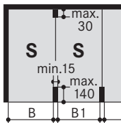
Single unit (2 cars)
